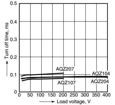
15.-(2) Turn off time vs. load voltage characteristics (Load voltage: 200, 400 V type) LED current: 10 mA; Continuous load current: 100 mA; Ambient temperature: 25°C 77°F
