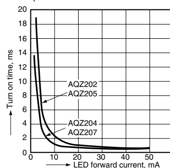
11.-(1) Turn on time vs. LED forward current characteristics (AC/DC type) Load voltage: 10 V (DC); Continuous load current: 100 mA (DC); Ambient temperature: 25°C 77°F
