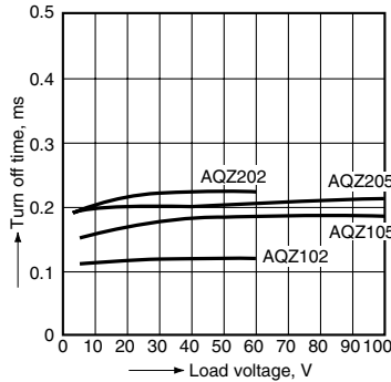
15.-(1) Turn off time vs. load voltage characteristics (Load voltage: 60, 100 V type) LED current: 10 mA; Continuous load current: 100 mA; Ambient temperature: 25°C 77°F
