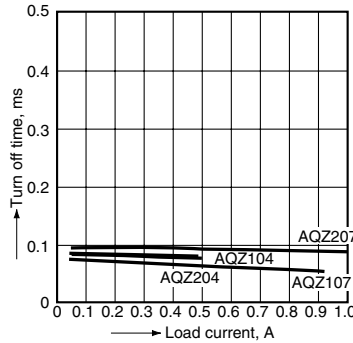
16.-(2) Turn off time vs. load current characteristics (Load voltage: 200, 400 V type) LED current: 10 mA; Load voltage: 10 V (DC); Ambient temperature: 25°C 77°F
