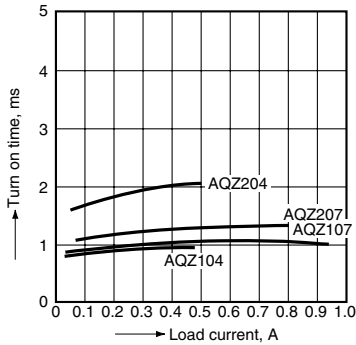
14.-(2) Turn on time vs. load current characteristics (Load voltage: 200, 400 V type) LED current: 10 mA; Load voltage: 10 V (DC); Ambient temperature: 25°C 77°F
